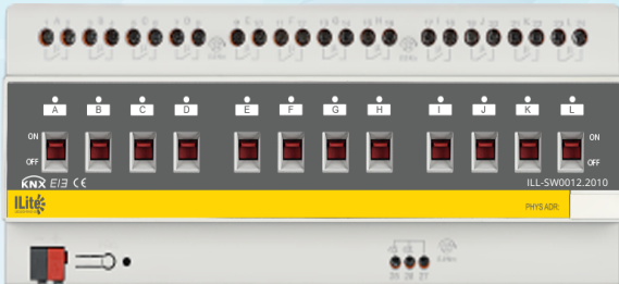
Switching Actuator 20A 12 Fold
